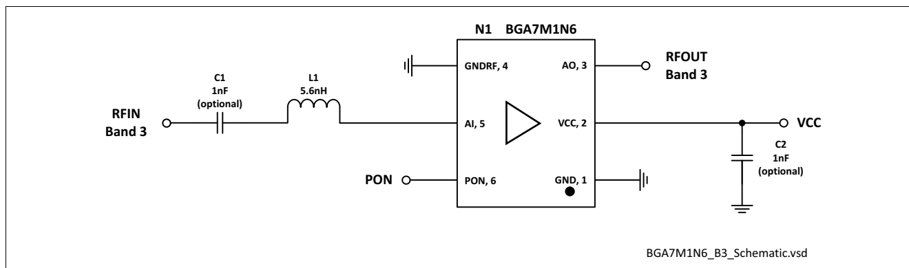
Figure 4 Application Schematic BGA7M1N6
