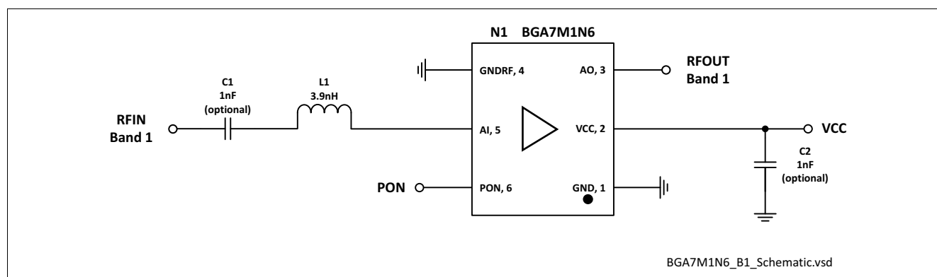
Figure 2 Application Schematic BGA7M1N6
