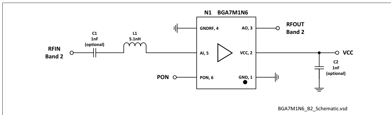
Figure 3 Application Schematic BGA7M1N6
